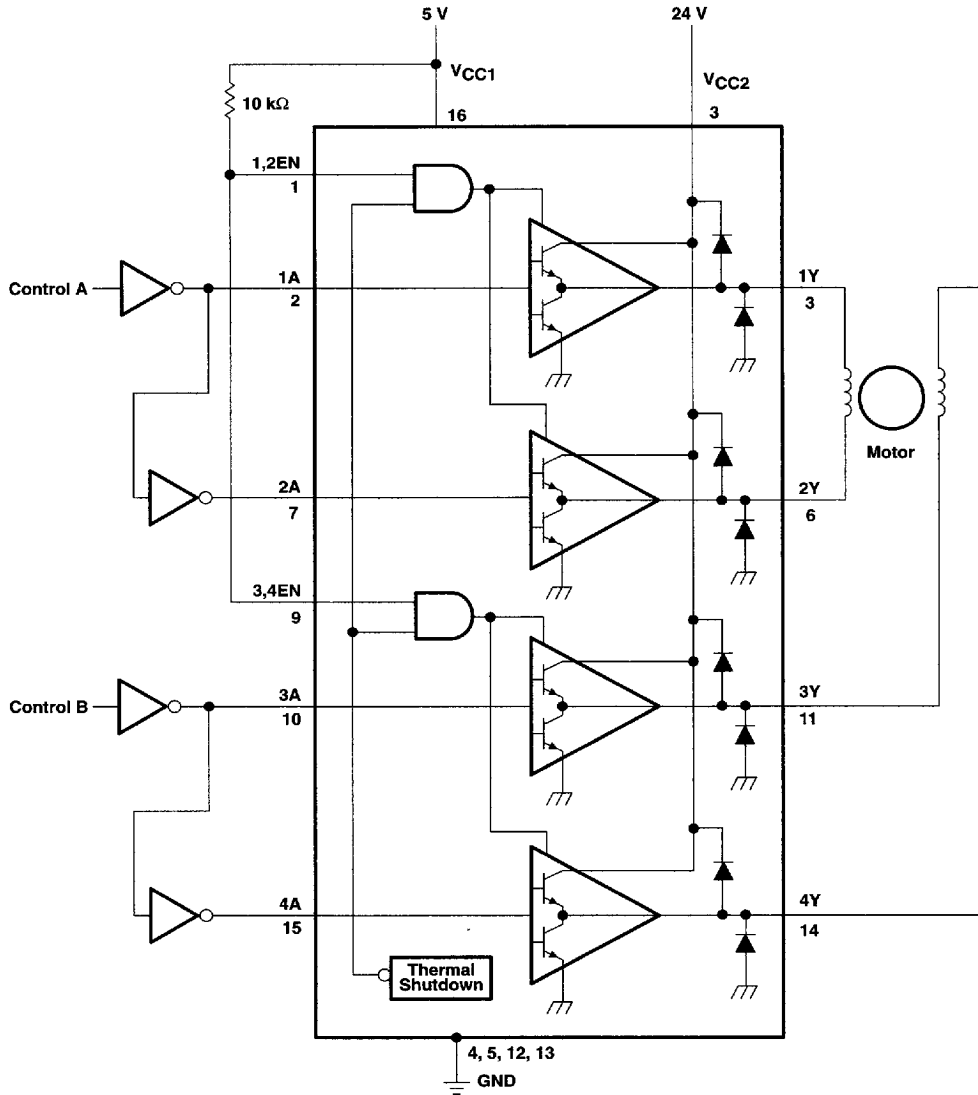
Figure 2. Two-Phase Motor Driver
